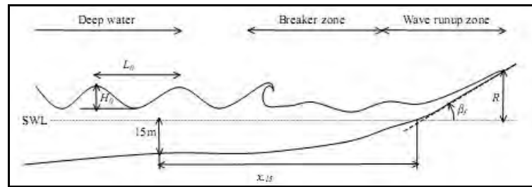
Figure 2. Showing parameters used in the model. R is the run-up value, x_{15} is the chart distance from the shoreline to the 15m isobath, H_0 is deep water significant wave height (taken from Mather et al. in press ).
